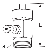
Measuring point For older STAD and STAF Max 150°C AMETAL®/EPDM
